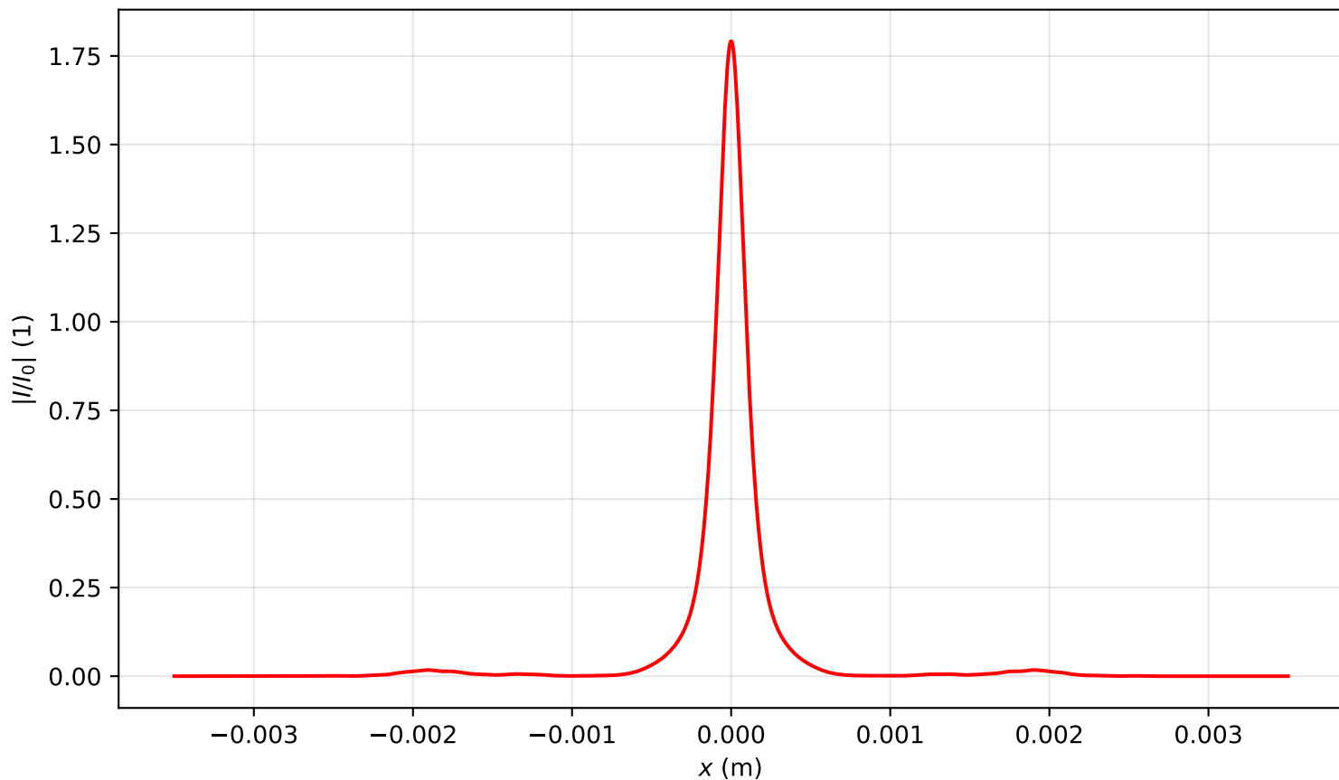
Intensity profile I(x, y = 0, z = 1.115)/I_0 , P_{in}=5.0P_{cr} , artificial time
